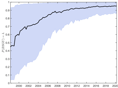
(c) \text{corr}(\zeta, v) = 0
