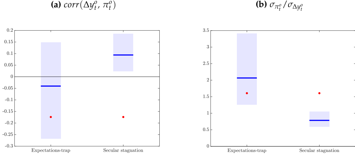
Figure 6: Moments: models vs data
